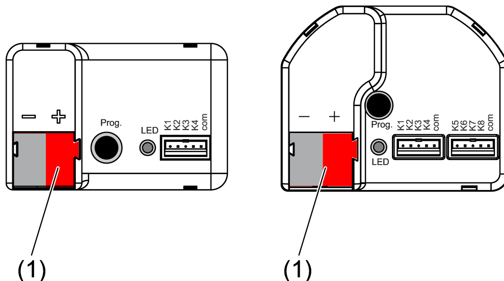
Figure 4: Bus connection
