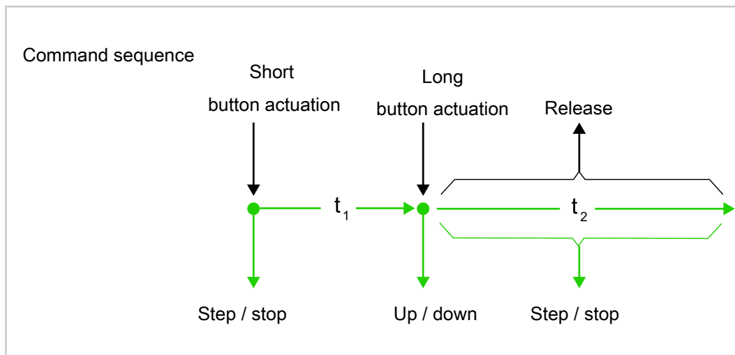
Figure 10: Operating concept "Step - Up/down - Step"
