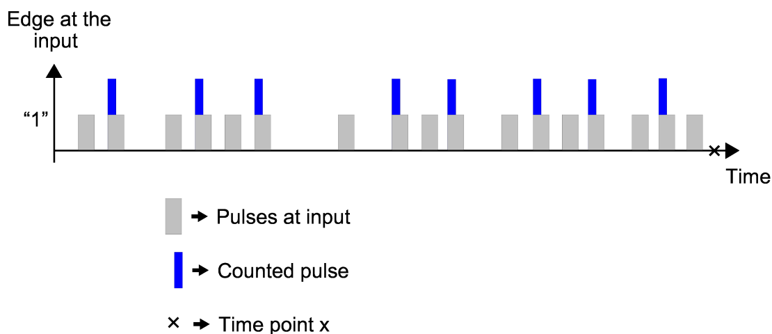
Figure 18: Example for setting the number of changes in counter status per counted pulse
